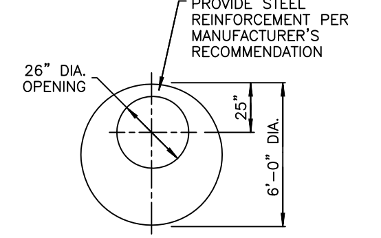
PRECAST CONCRETE TOP SLAB DETAIL
