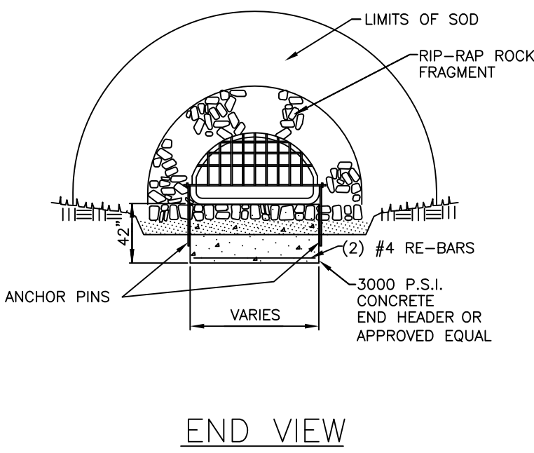
END VIEW
