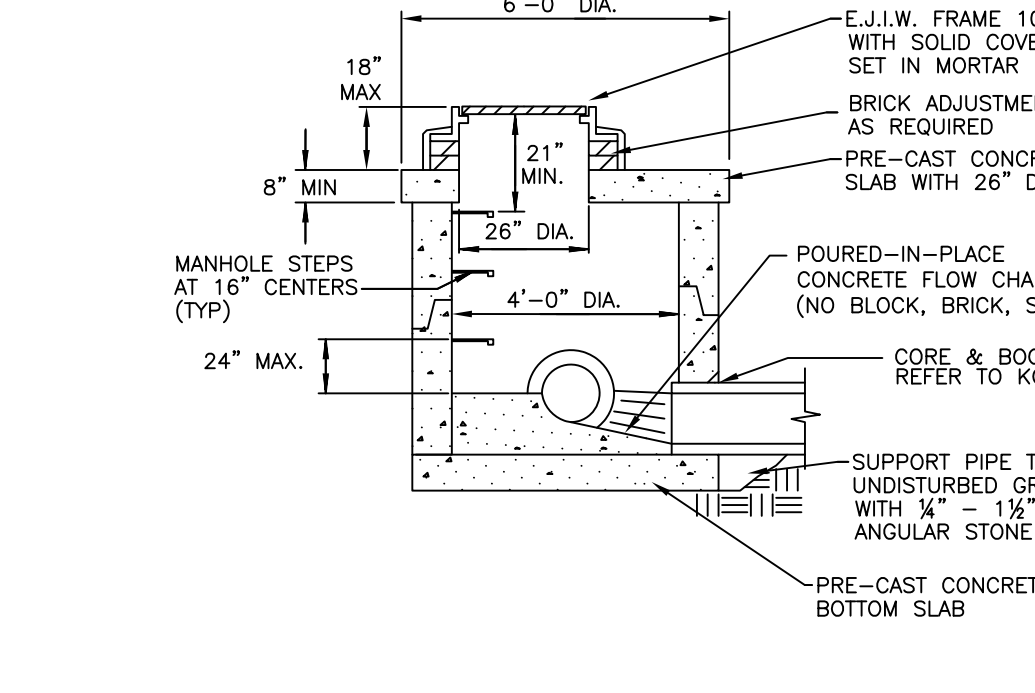
PRE-CAST LOW HEAD MANHOLE DETAIL NO SCALE (PRIOR APPROVAL ONLY)
